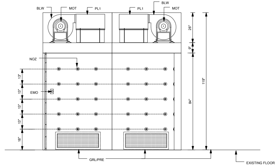
ELEVATION "A"
