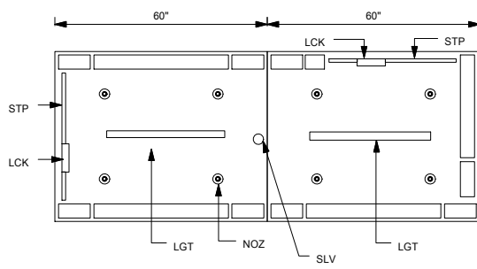
ROOF VIEW
