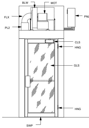
ELEVATION "A"
