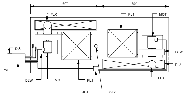
ROOF VIEW
