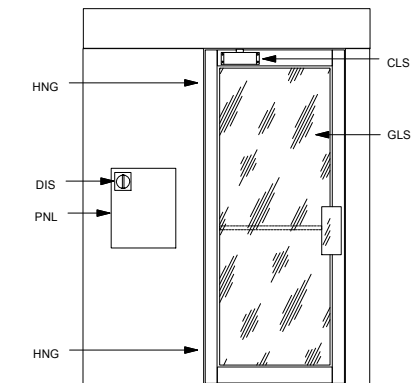
ELEVATION "A"
