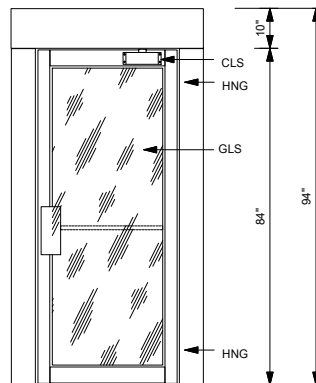
ELEVATION "D"
