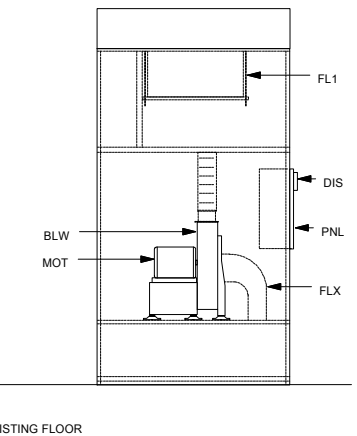
ELEVATION "B" cut away view
