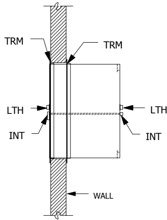
ELEVATION "B"
