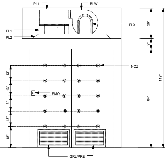
ELEVATION "D" CUTAWAY VIEW
