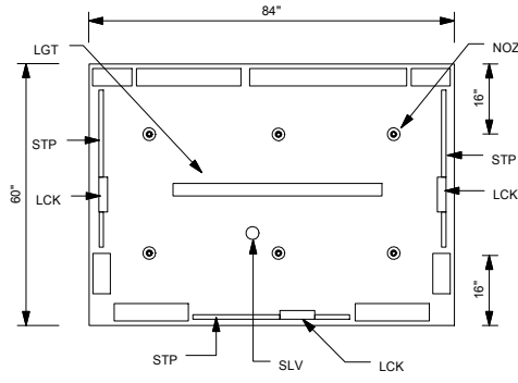
CEILING VIEW
