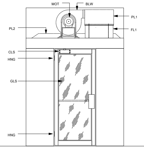
ELEVATION "B"
