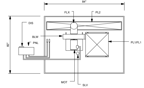
ROOF VIEW
