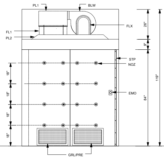
ELEVATION "D"
