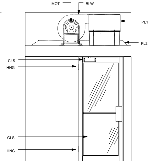
ELEVATION "B"
