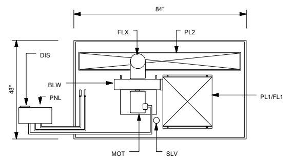
ROOF VIEW
