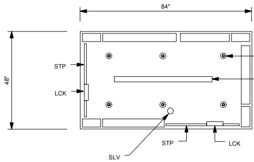
CEILING VIEW
