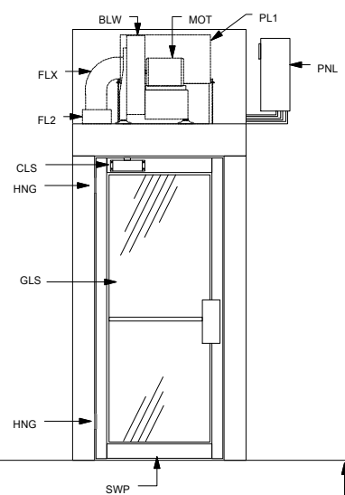
ELEVATION "A"
